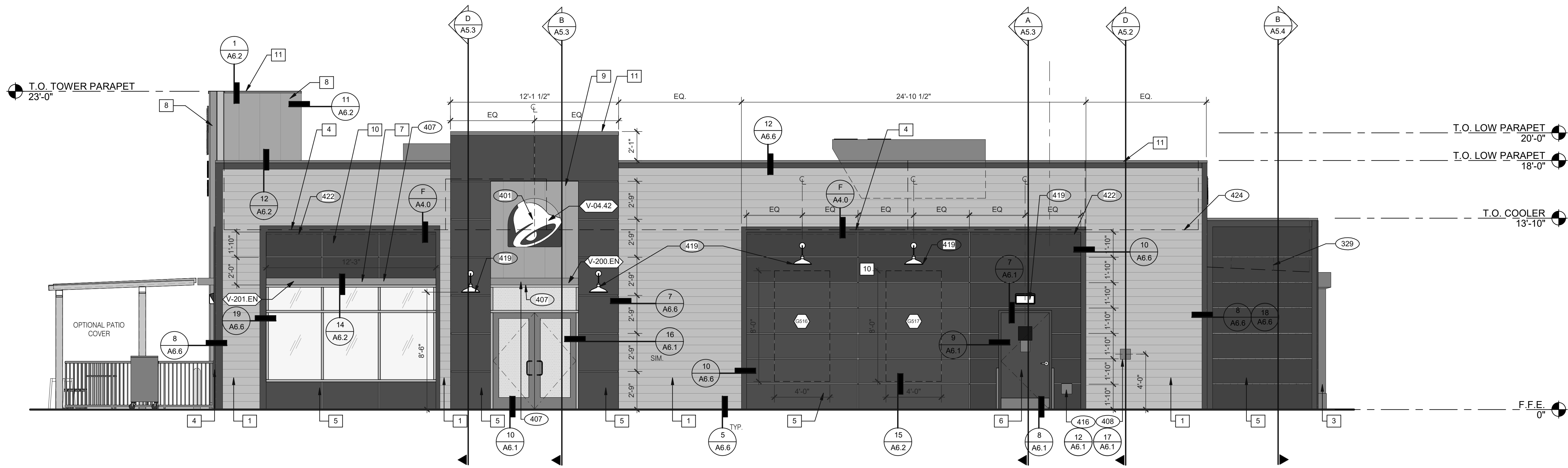
FRONT ELEVATION 1/4" = 1'-0" 1
