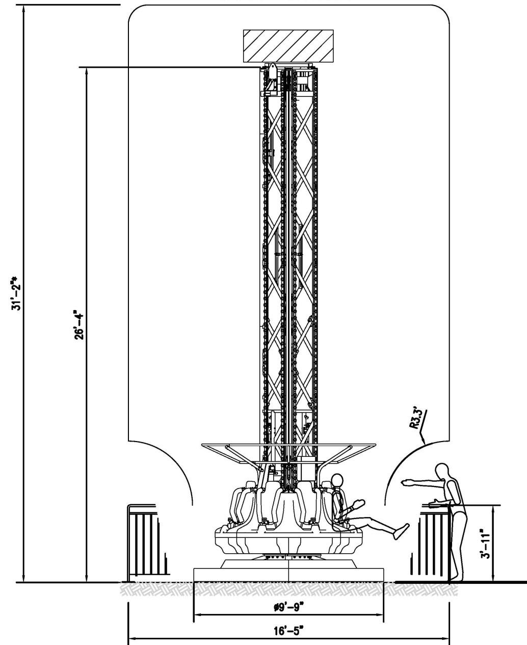
AIR TOWER (8 SEATS) (NOT TO SCALE)
