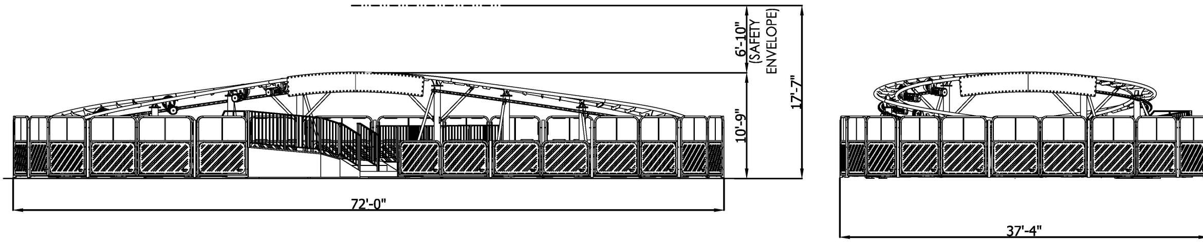
SPINNING COASTER 2.0 ELEVATIONS (NOT TO SCALE)
